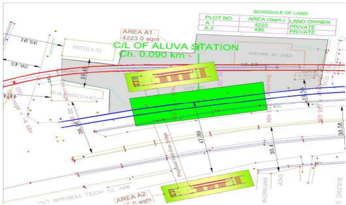
Figure 5.6.3: Proposed Aluva Station Area Development Plan
